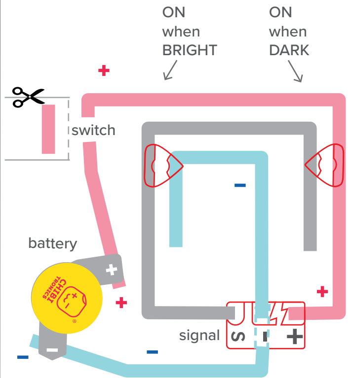
LIGHT SENSOR WITHOUT A MICROCONTROLLER
