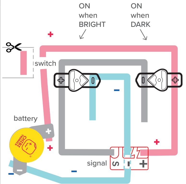
LIGHT SENSOR WITHOUT A MICROCONTROLLER
