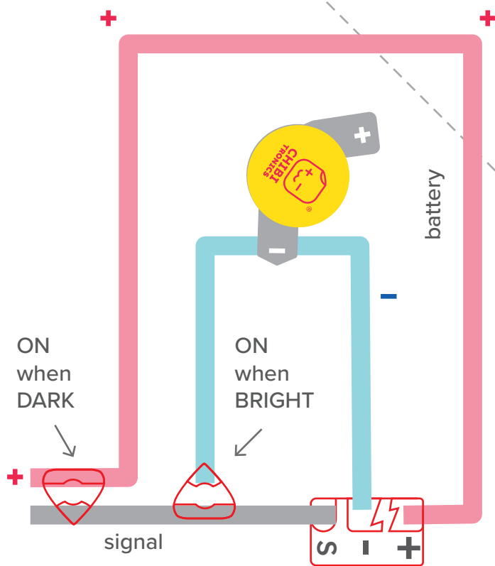
LIGHT SENSOR WITHOUT A MICROCONTROLLER
